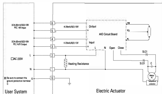
AC 220V Modulating type Wiring diagram
