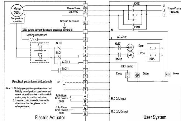
AC380V Standard On/Off Type Wiring diagram
