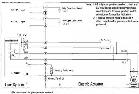
On/Off Type AC220V
