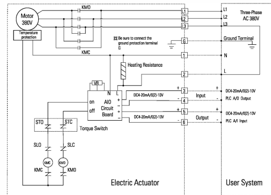
Three-Phase AC 380V Modulating type Wiring diagram
